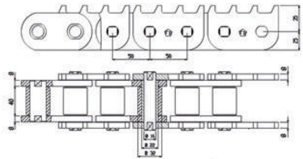
LZK40.50FB-50x8
