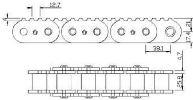
LEK120-1T
